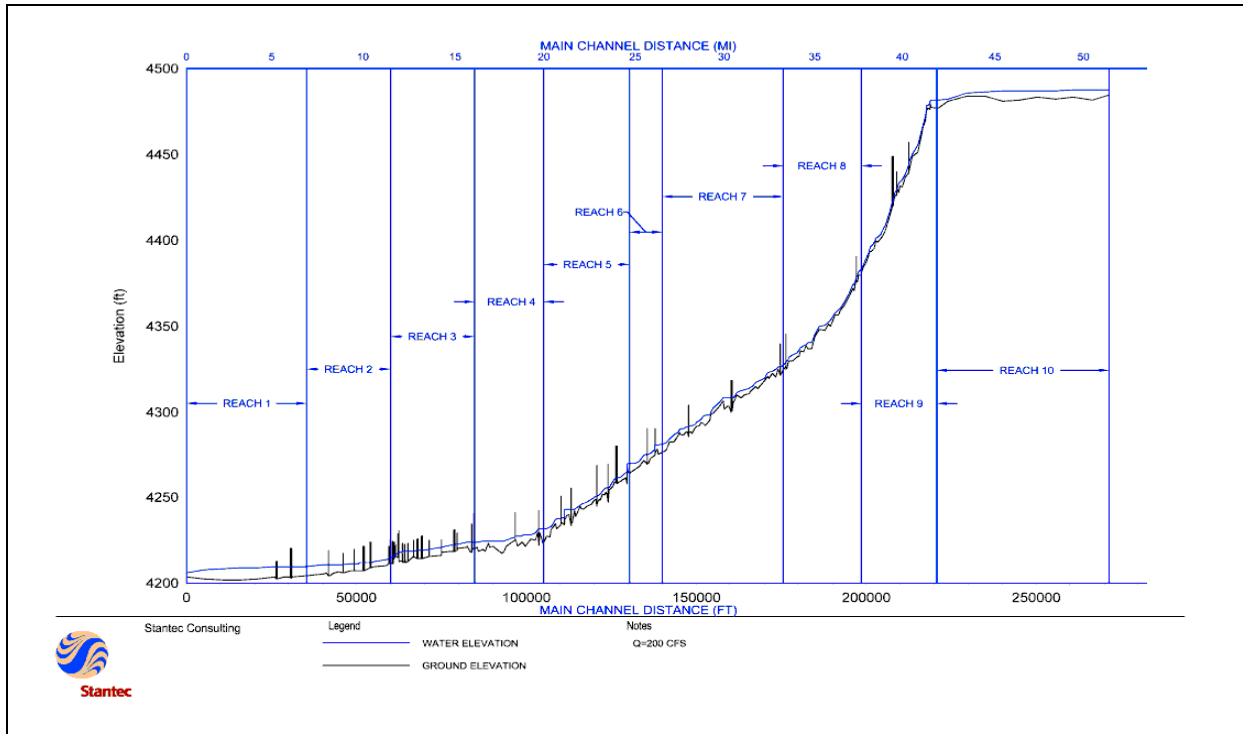
Figure D.3. Jordan River elevations (Reaches 1–3 are the same as DWQ Segments 1–3 and correspond to the lower Jordan River from Burton Dam upstream to 2100 South) (Reproduced from Figure 4-3 in Stantec 2006a.)
